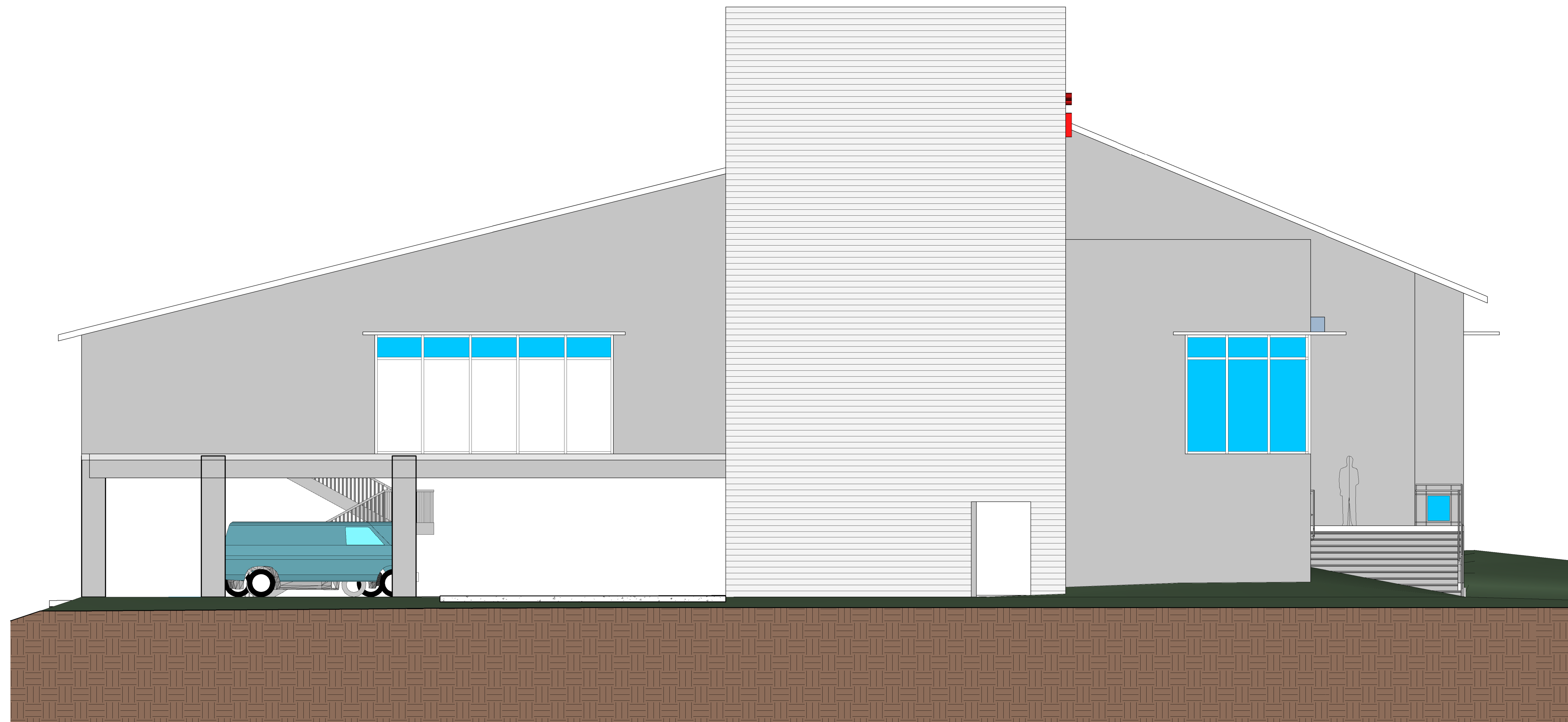
1 WEST ELEVATION A301P 3/16" = 1'-0"
